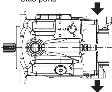
Side ports
