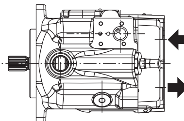
Rear ports
