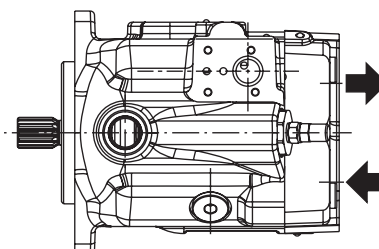
Rear ports
